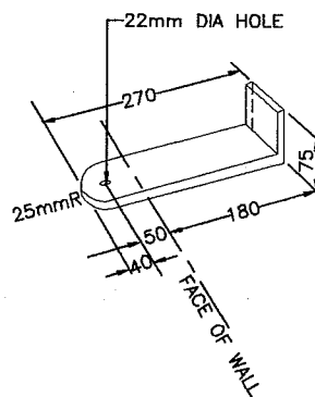
12mm x 50mm FLAT BAR
