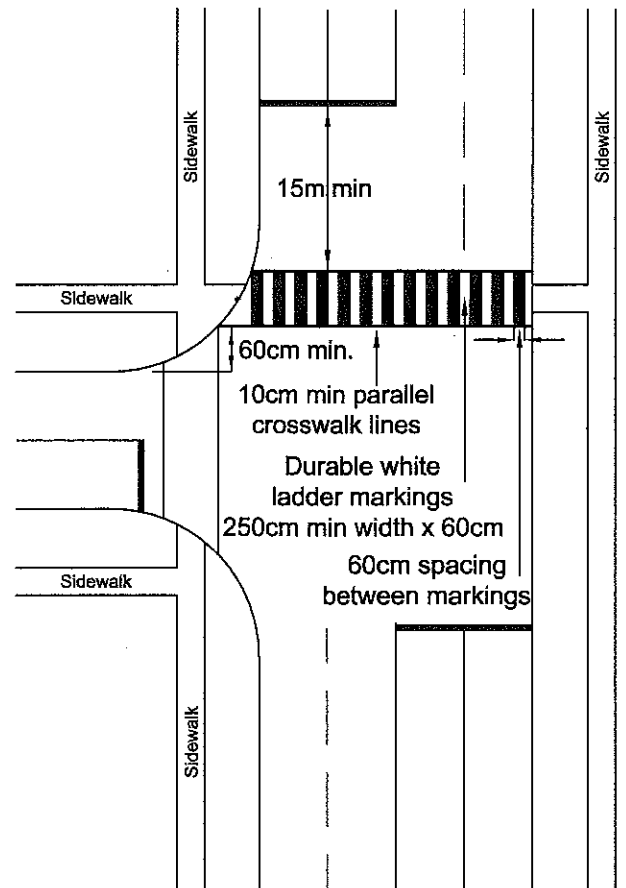
TYPICAL INTERSECTION PEDESTRIAN SIGNAL
