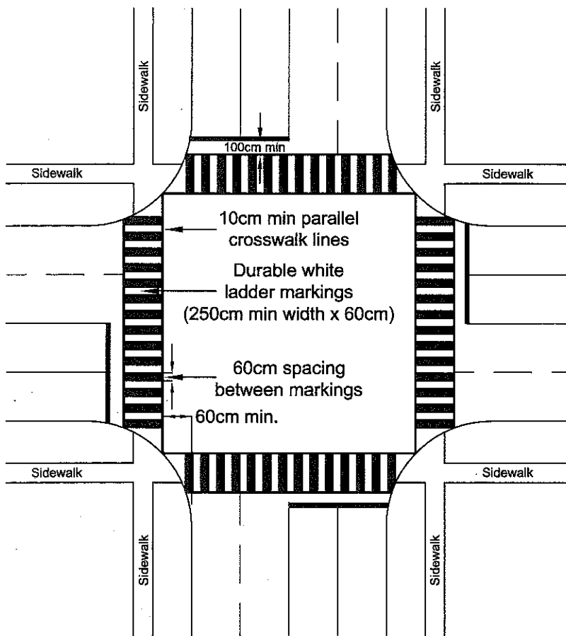
TYPICAL SIGNALIZED INTERSECTION
