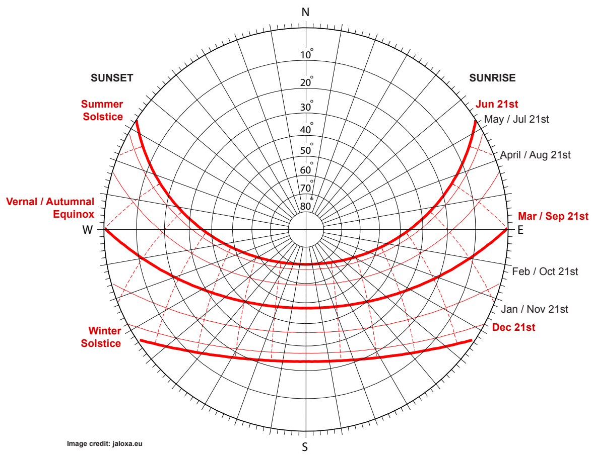
Figure 3.1 - Sterographic Sunpath Diagram (Latitude 43N)
