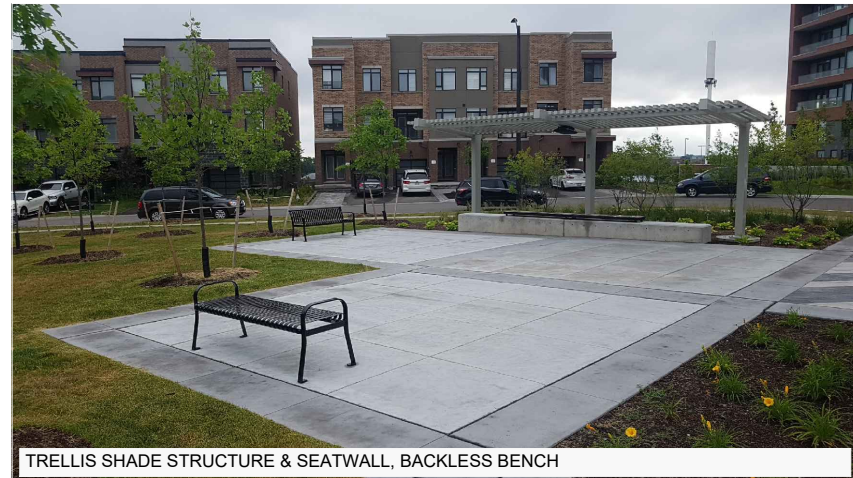
TRELLIS SHADE STRUCTURE & SEATWALL, BACKLESS BENCH
