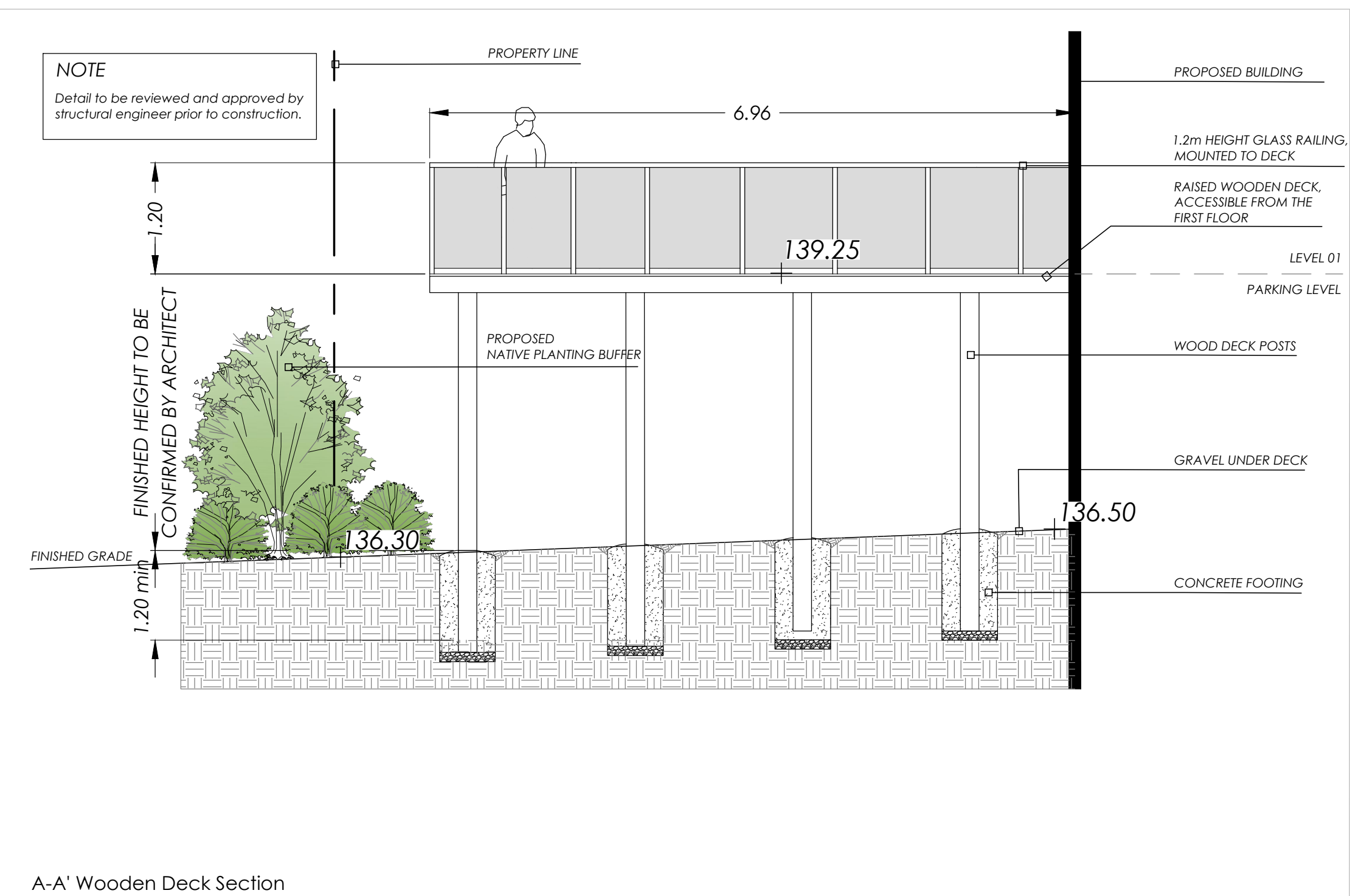
A-A' Wooden Deck Section
