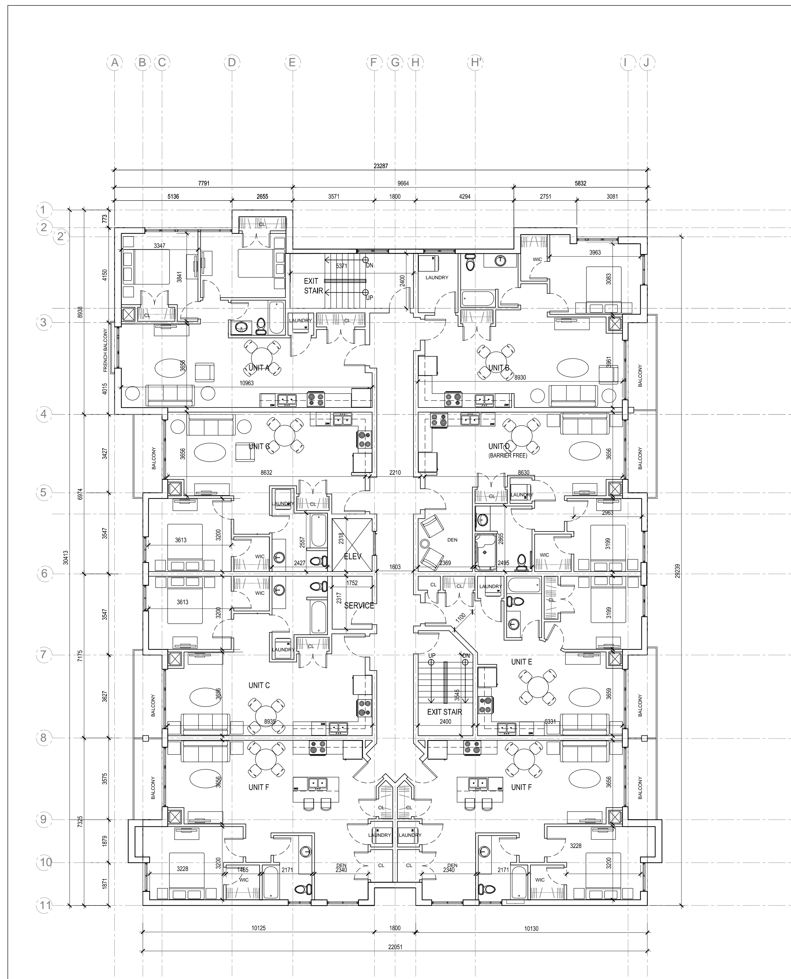
1 SECOND AND THIRD FLOOR 1 : 100
