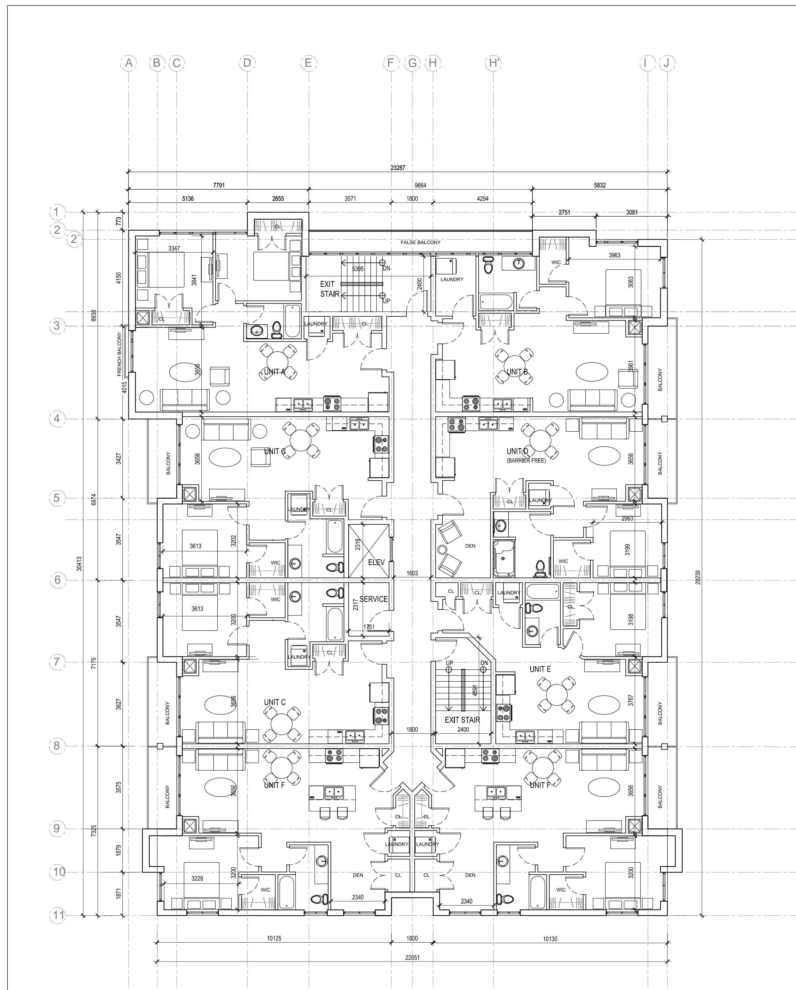
2 FOURTH FLOOR 1 : 100
