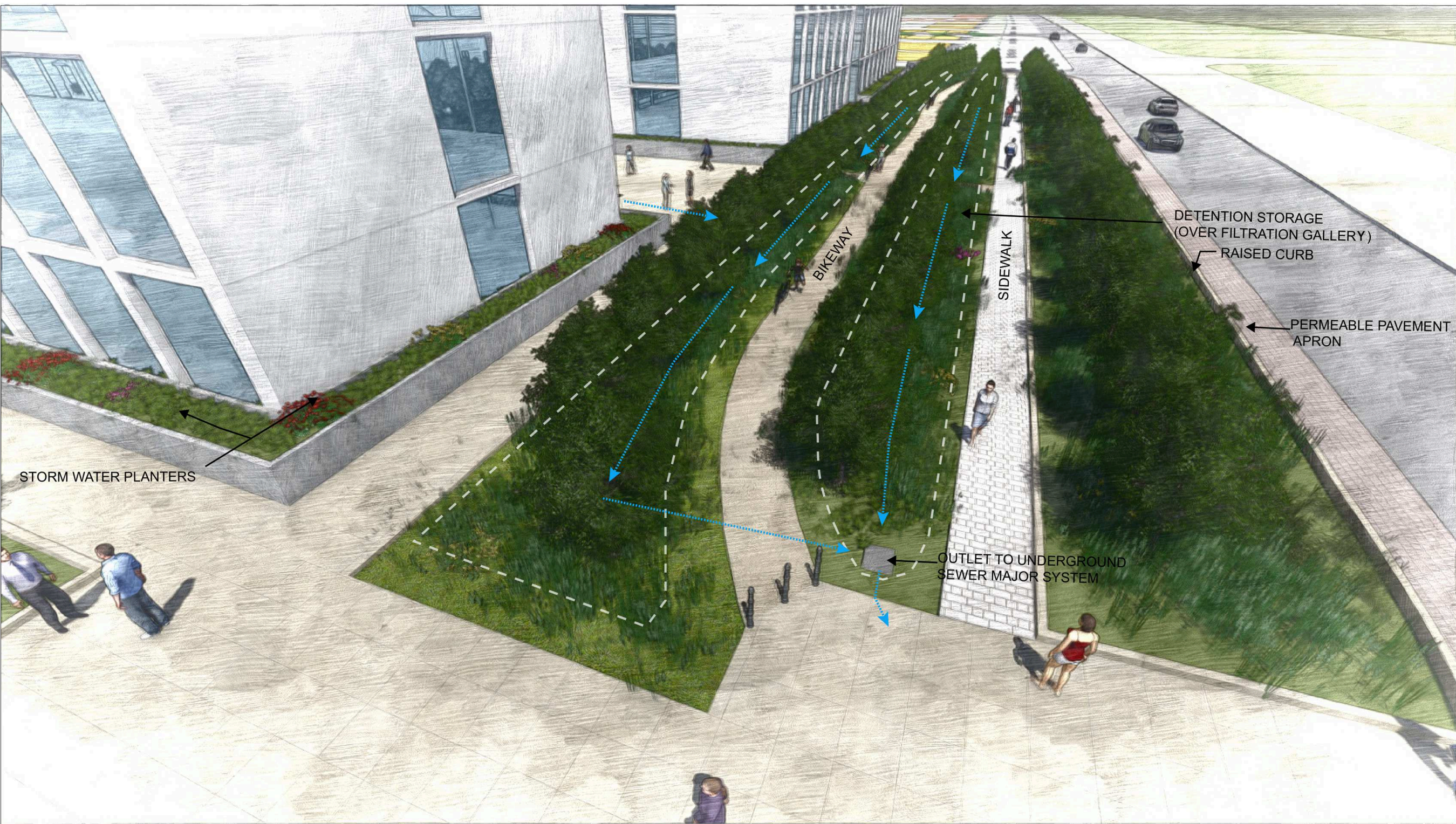
LID Options: 'Greenway' along Tremaine Road frontage of the site
